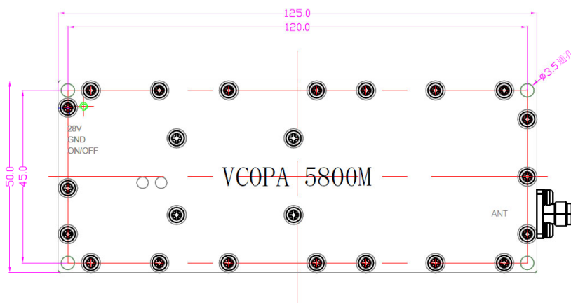
3000-5900MHz Deawing
