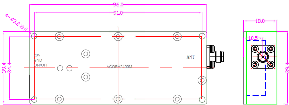
1100-2700MHz Deawing
